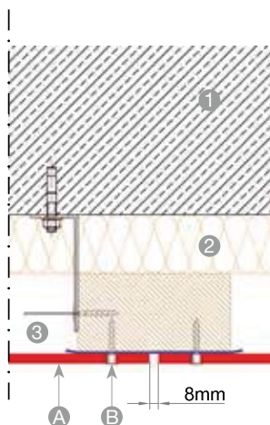
JOINT VERTICAL
