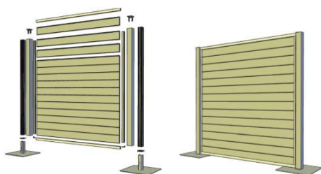
Tecnodeck Fence System 2x2 Light Version: Not fixed, with base plate
