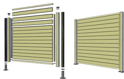
Tecnodeck Fence System 2x2 Light Version: Fixed base
